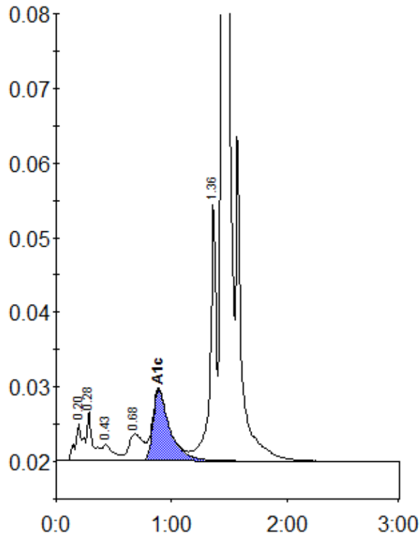
Peak table - ID: 10415914
